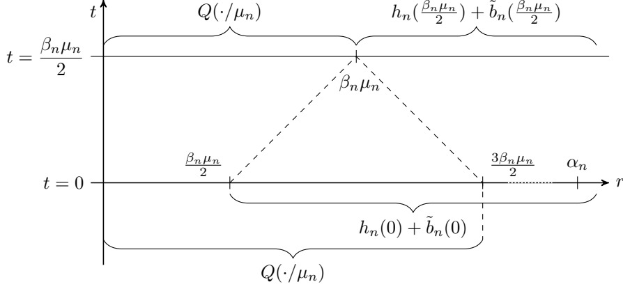
FIGURE 2. A schematic description of the evolution of the decomposition (3.74) from time t = 0 until time t = \frac{\beta_n \mu_n}{2} . At time t = \frac{\beta_n \mu_n}{2} the decomposition (3.85) holds.
