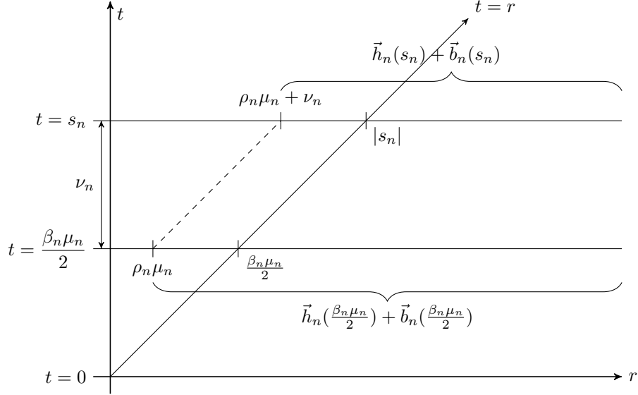
FIGURE 3. A schematic depiction of the evolution of the decomposition (3.85) up to time s_n . On the interval [s_n, +\infty) , the decomposition (3.87) holds.
