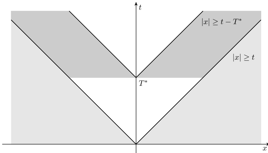
FIGURE 1. Exterior region without and with time delay
