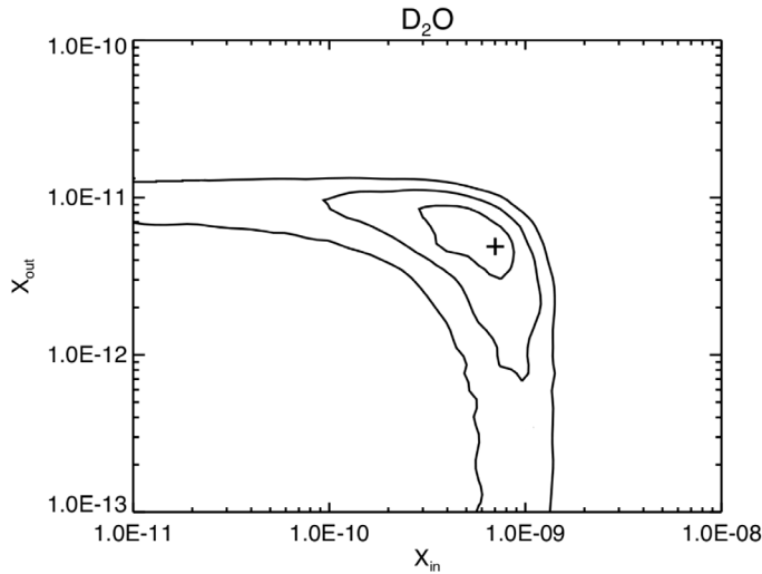
Fig. 3. \chi^2 contours at 1 \sigma , 2 \sigma , and 3 \sigma obtained when adding an absorption layer with a para-D 2 O column density of 1.1 \times 10^{12} \text{ cm}^{-2} and ortho-D 2 O column density of 1.4 \times 10^{12} \text{ cm}^{-2} . The best-fit model is represented by the symbol “+”.
