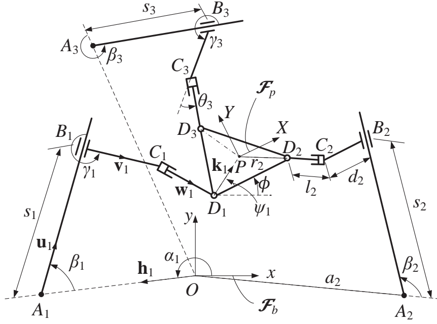
Fig. 2 Parameterization of the 3-PPR PPM.
