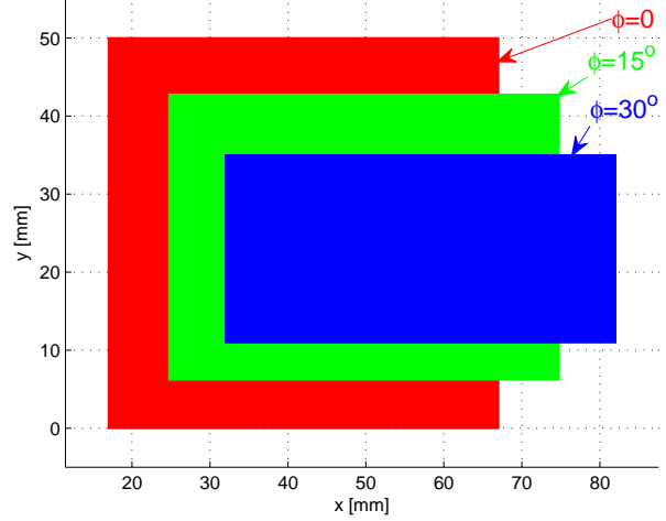
Fig. 3 Constant-orientation workspaces.
