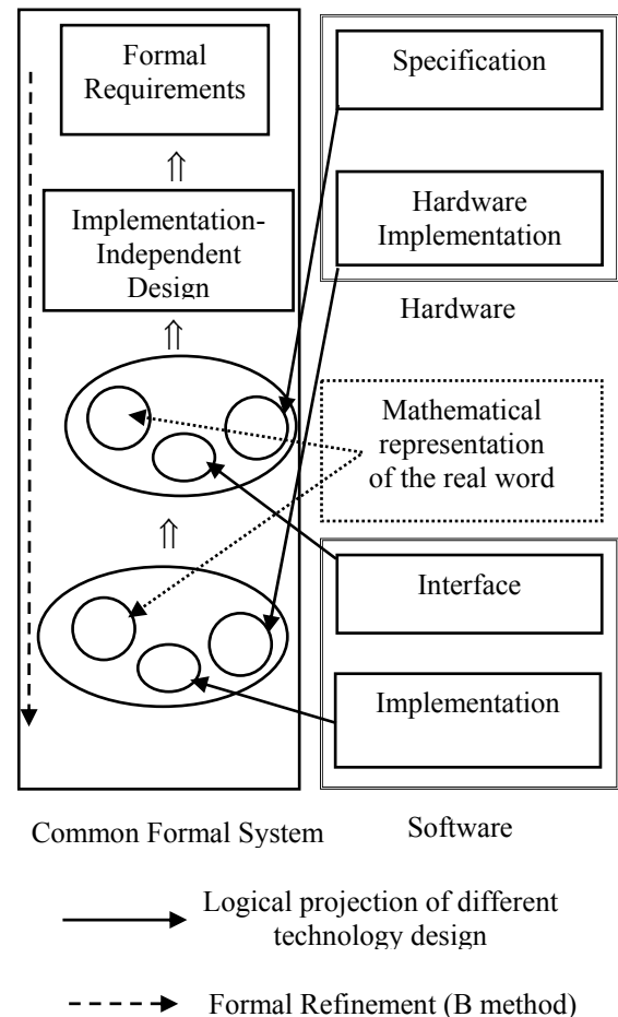
Figure 1: Refined MDA
