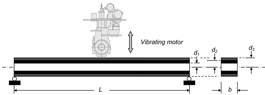
Figure 7 – Engine support platform.
