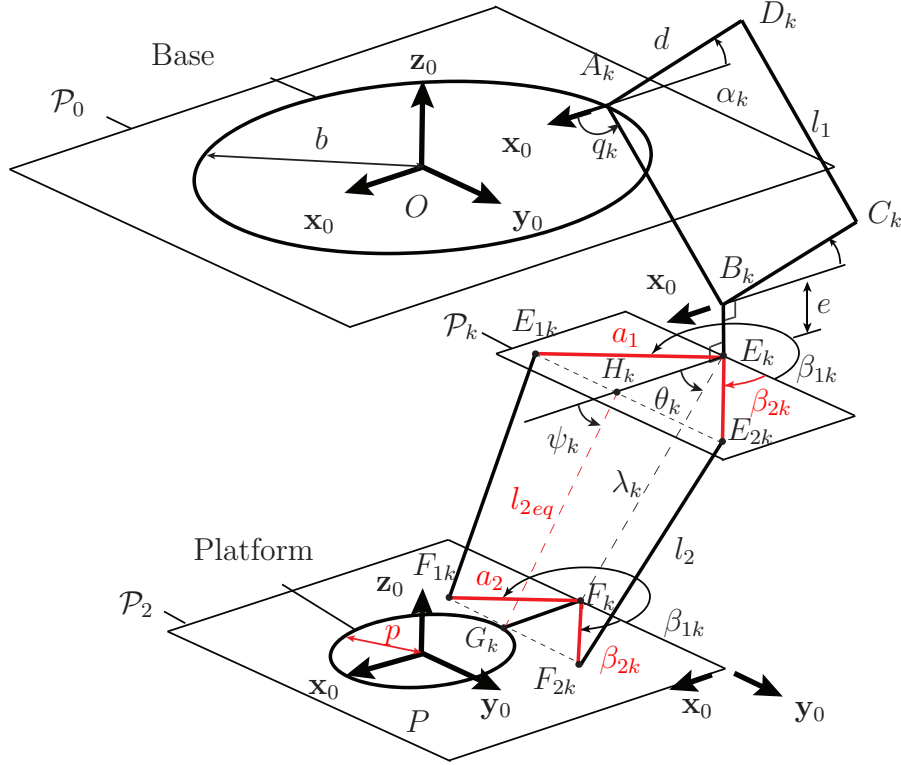
Figure 3: Paramaterization of the k th leg ( k = I, II )
