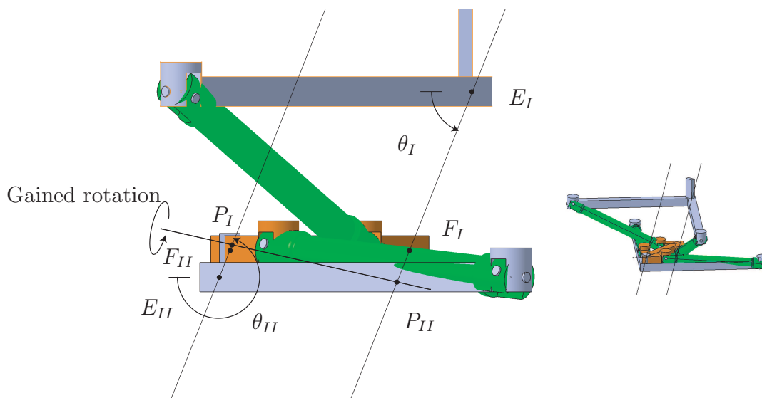
Figure 11: Front view of the distal loop of the IRSBot-2 in a constraint singular configuration corresponding to Case II ( \theta_{II} = \theta_I + \pi )
