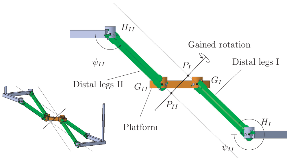
Figure 10: Front view of the distal loop of the IRSBot-2 in a constraint singular configuration corresponding to Case I ( \psi_{II} = \psi_I + \pi )
