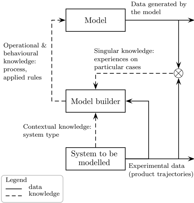
Fig. 1. Data and knowledge flow from/to the model builder
