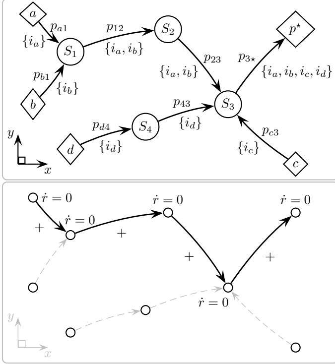
Fig. 2. Example of the directed graph of a product p^* . Top: the diamonds represent the birth or disappearance of objects and/or products. The circles represent operations. Labels associated with arrows represent the product and all associated product identifiers at each level of the process of transformation. Bottom: speed of component a
