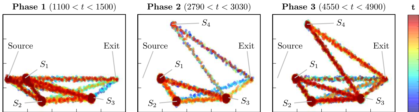
Fig. 4. Model adaptation. Phase 1: The system consists of three servers. Phase 2: Emergence of a new server. Phase 3: The new server is validated.
