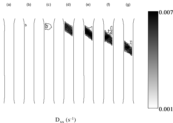
Figure 6: Distribution of the D_{xx} component of the strain-rate tensor during longitudinal propagation of a Lüders band
