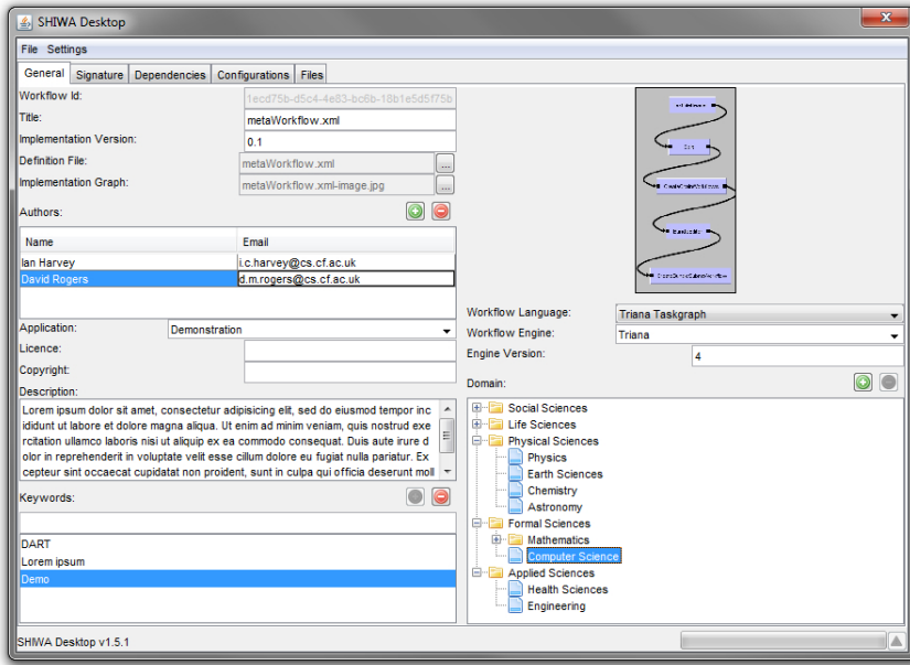
Fig. 7: SHIWA Desktop GUI
