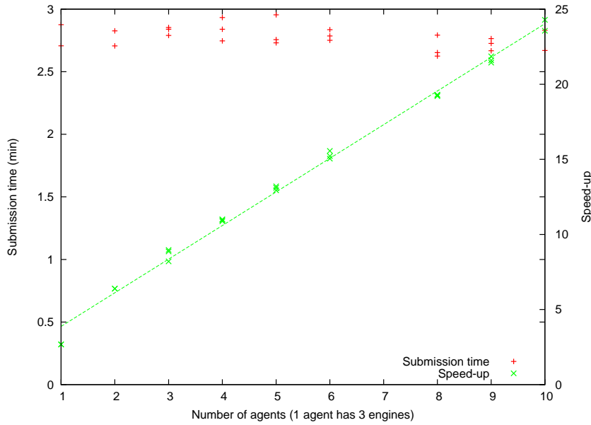
Fig. 9: Evaluation of the pool scalability, w.r.t the number of available agents
