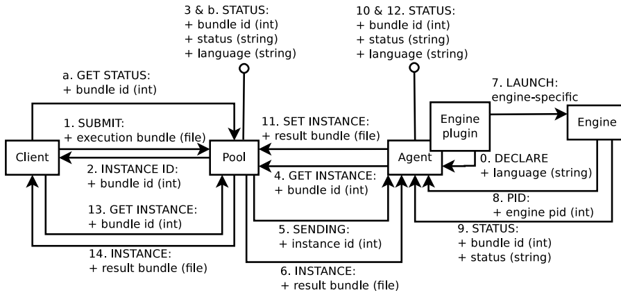
Fig. 5: Interactions between client, pool, agent, and engine.
