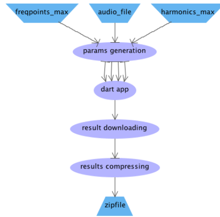
Fig. 10: DART Music Information Retrieval (MIR) workflow
