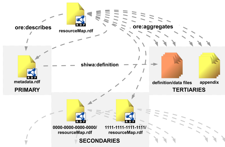
Fig. 1: Anatomy of an Aggregation in a SHIWA Bundle
