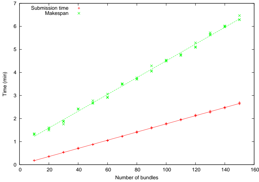
Fig. 8: Evaluation of the pool scalability, w.r.t the number of concurrent active bundles
