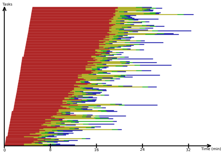
Fig. 11: Jobs timeline of DART application on the EGI
