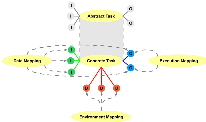
Fig. 2: Bundle Metadata Structures and their interactions
