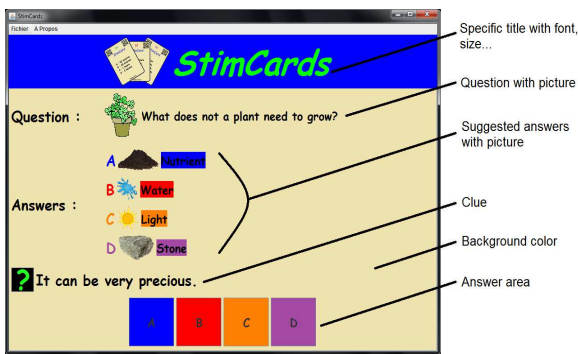
Figure 2. A loaded card in StimCards GUI
