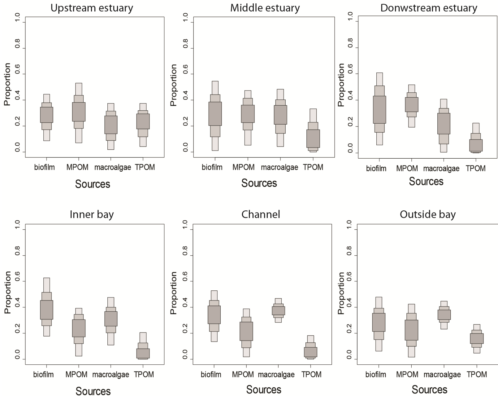
Figure: composition of Suspended Particulate Organic Matter (SPOM) by SIAR analysis along the gradient. MPOM=marine POM, TPOM=terrestrial POM. Values of sources were the same used in oyster diet modeling (Fig. 5 in the manuscript)
