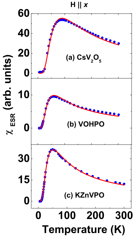
FIG. 6. (Color online) Full circles: temperature dependence, for 4.2 \leq T \leq 300 K, of the corrected static susceptibility of (a) \text{CsV}_2\text{O}_5 , (b) \text{VO}(\text{HPO}_4) \cdot 0.5\text{H}_2\text{O} , and (c) \text{KZn}(\text{H}_2\text{O})(\text{VO})_2(\text{PO}_4)_2(\text{H}_2\text{PO}_4) , as deduced from the ESR measurements for H parallel to the x direction, after subtraction of the susceptibility of impurities. Continuous curves: fits of the experimental data to the theoretical temperature dependence of spin- \frac{1}{2} dimer systems as expressed by Eq. (1).
