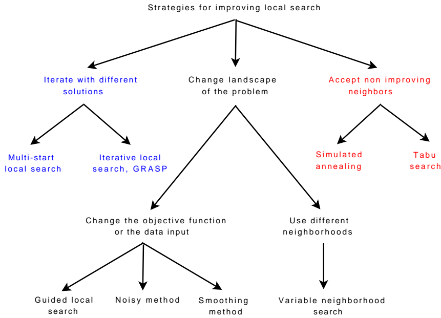
Fig. 2 Local search family of algorithms for the improvement of hill-climbing and escaping from local optima.
