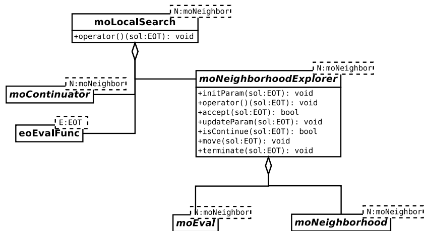
Fig. 6 Simplified UML diagram for the design of local search algorithms.
