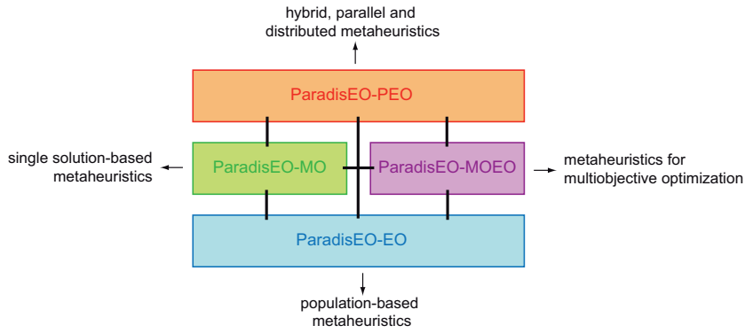
Fig. 5 Interacting modules of the ParadisEO software framework.
