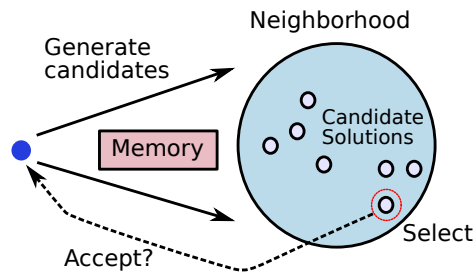
Fig. 1 Template for local search metaheuristic: (i) generate candidate solutions from the neighborhood, (ii) select a neighbor, (iii) decide to replace the current solution by the selected neighbor.
