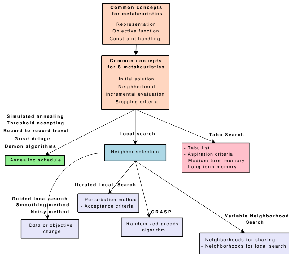
Fig. 4 Common concepts and relationships in local search metaheuristics.
