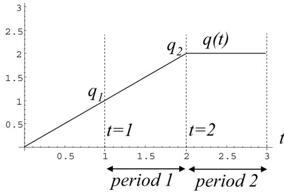
Figure 1 – Representation of the quality over time of SaaS software with Vidyand Choudhary’s model
