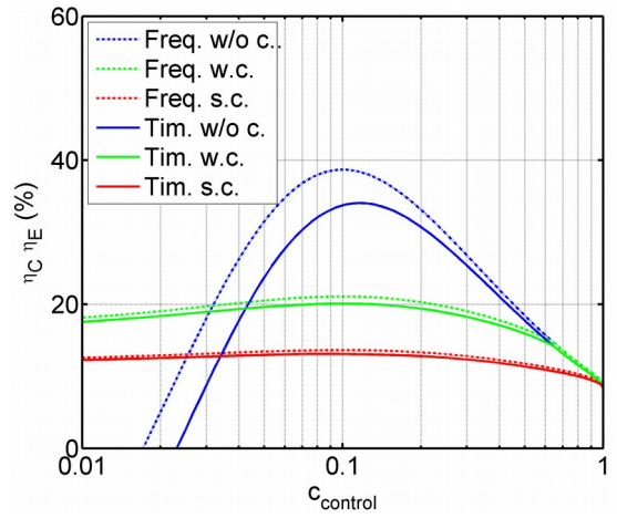
Fig. 10. Global efficiency as a function of control parameter c_{control} for T_p = 9.5 s under the hypothesis c_{loss} = 0.10 . The Global efficiency is the product of the control efficiency \eta_c and the electric efficiency \eta_e . Solid lines represent the time-domain simulation and dashed lines the approximation in the frequency domains. Blue lines correspond to the solutions without stability constraints (w/o c.), green lines with weak stability constraints (wc) and red lines with strong stability constraints (sc).
