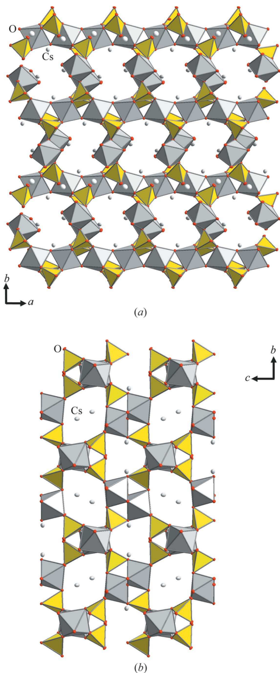
Figure 2 Projections along (a) the [001] direction and (b) the [100] direction of (I), showing the vanadium octahedra (grey in the electronic version of the paper), the phosphate tetrahedra (yellow), the O atoms (red) and the \text{Cs}^+ cations (white) in the channels.
