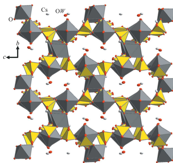
Figure 3 Projection along the [100] direction of (II), showing the vanadium octahedra (grey in the electronic version of the paper), the phosphate tetrahedra (yellow), the O atoms (red) and the \text{Cs}^+ cations (white) in the channels together with water molecules.
