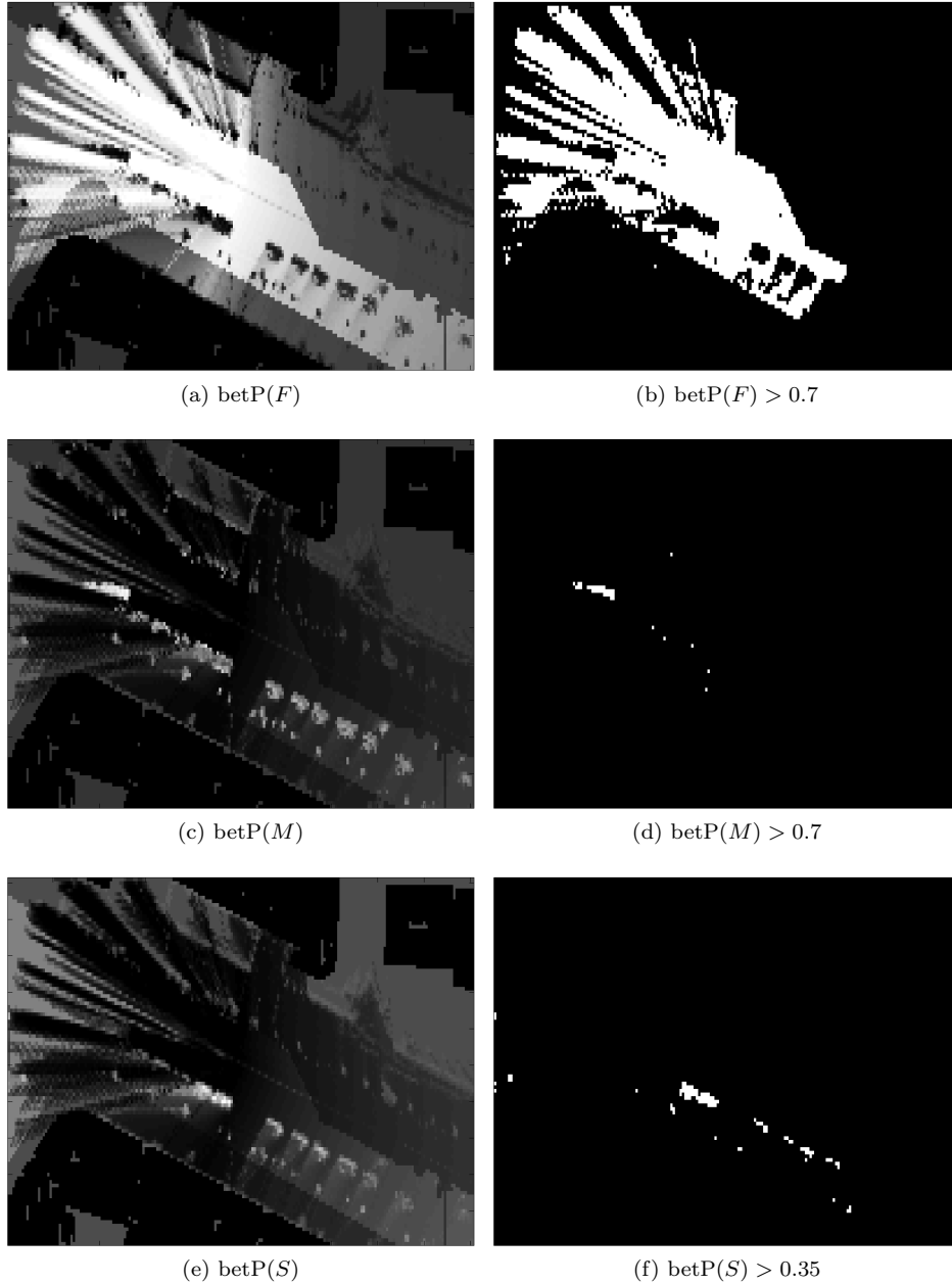
Figure 15: PerceptionGrid. Left column: pignistic probability ( \text{betP} ) for different classes. Right column: a simple decision rule example – threshold on pignistic probability.
