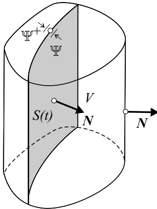
FIGURE 2. Singular surface
