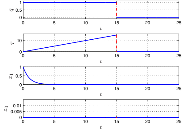
(b) Controller trajectory
