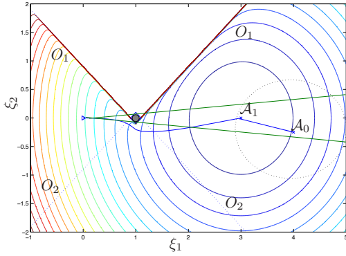
(a) Plant trajectory with initial conditions \xi(0,0) = 0 , q(0,0) = 1 , \zeta_1(0,0) = 1 , steered below the obstacle using \kappa_1(\xi, 1) while in \zeta_1 = 1 .
