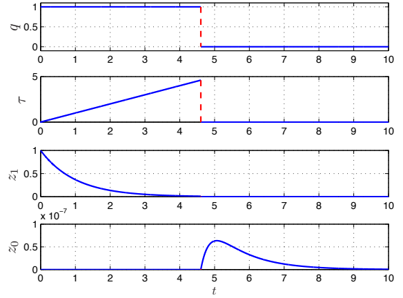
(b) Controller trajectory
