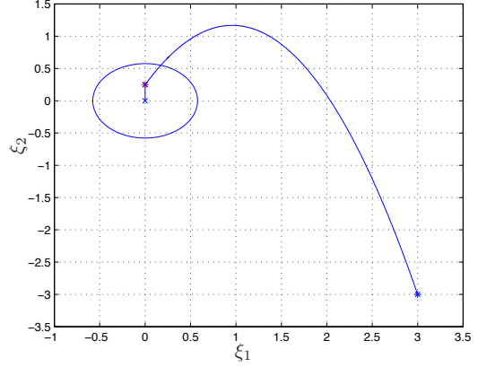
(a) Plant trajectory
