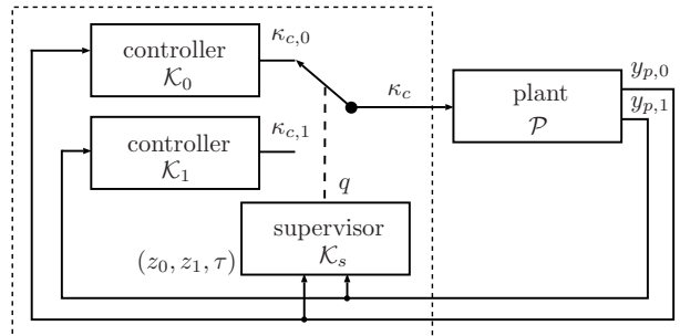
Fig. 1. Proposed control approach for Problem (\star) .
