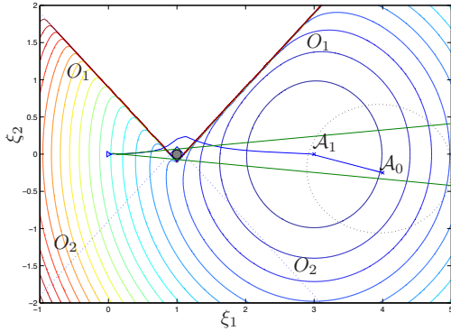
(b) Plant trajectory with initial conditions \xi(0,0) = 0 , q(0,0) = 1 , \zeta_1(0,0) = 2 , steered above the obstacle using \kappa_1(\xi, 2) while in \zeta_1 = 2 .
