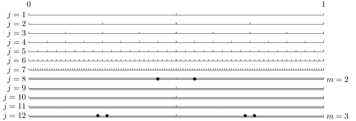
Figure 2: Case \beta = 2 and \alpha = 2 . The non vanishing wavelet coefficients \bullet appear on dyadic points \frac{k}{2^j} = \frac{K}{2^{m-1}} \pm \frac{1}{2^{\alpha m}} with K odd and j = \alpha \beta m .
