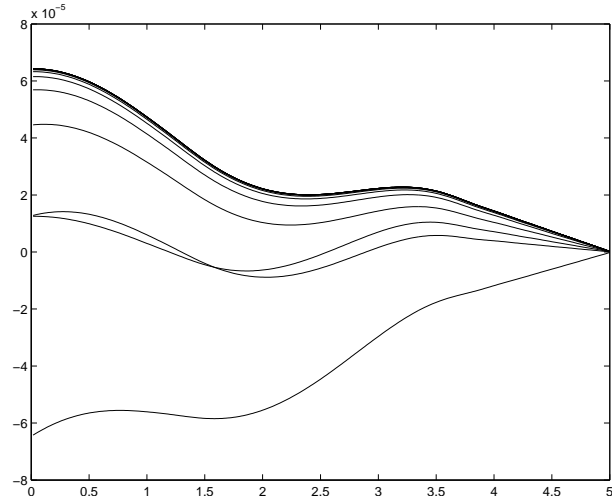
FIG. 4.3. Functions \psi_1(t, ., \xi_l) l = 1 : L at time t = 1.3 \text{ ms}
