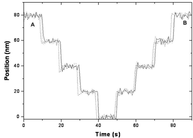
FIG. 7. Position step of 20 nm corresponding to different ellipticity values. (a) Straight curve \varepsilon=0 . (b) Dotted curve \varepsilon=5^\circ . (c) Dashed curve \varepsilon=10^\circ . The effect of a residual ellipticity of the laser beam polarization state is canceled out by the effect of the filtering of the second harmonic.
