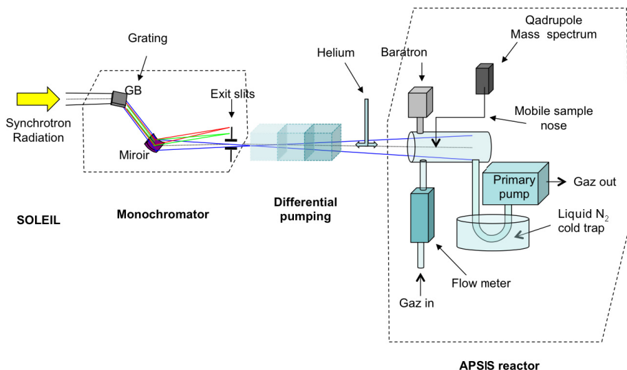
Fig. 1. Principle of the Atmospheric Photochemistry Simulated by Synchrotron (APSYS) set up and its coupling with the APEX branch of the DISCO beamline.
