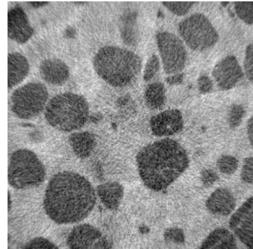
Fig. 1. Material A; size: 500 \times 500 \times 150 ; resolution: 3 \mu\text{m} .
