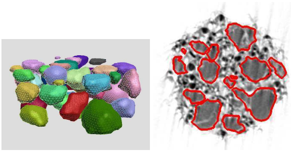
Fig. 9. First image: the 3D mesh on a segmented image of material B. Second image: a slice of the segmented image. The red lines represent the numerical grains boundary and match the visual segmentation.
