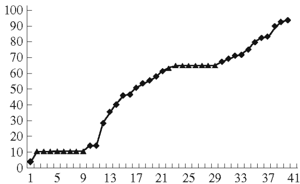
Fig. 4. Distribution of the eigenfrequencies of the big system: the eigenfrequencies of (▲) an individual nanocrystal and (◆) the substrate.
