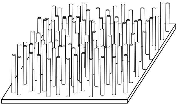
Fig. 1. Big system: an array of nanocrystals or nanotubes on a substrate.
