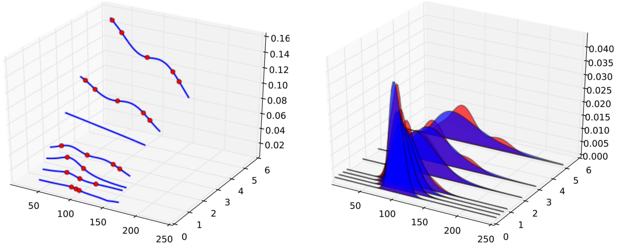
Figure 5: Arbitrage-free calibration of 7 Radon-Nikodym densities from sparse vanilla option data. The forward price is 100. On the left-hand side, we plot the sequence of implied total lognormal variances (input data and interpolation). The right-hand side shows the superimposition of the calibrated risk-neutral densities and base model's densities (Black-Scholes) for the same 7 maturities. The 4th maturity in the calibration does not have any listed option price.
