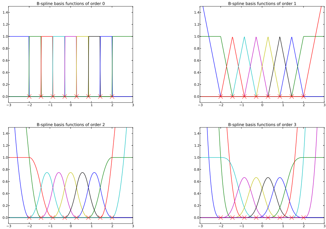
Figure 1: The B-spline basis functions of order 0, 1, 2 and 3, corresponding to the same given set of 8 knots.
