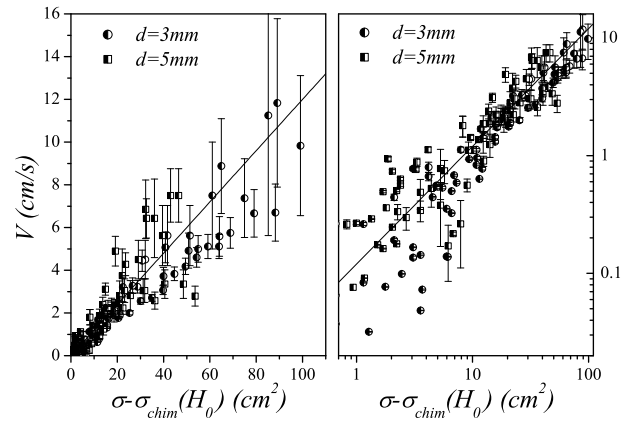
FIG. 10. Expansion rate V = H_0/T plotted versus \sigma - \sigma_{chim}(H_0) in linear-linear and log-log representations for all the data obtained with bead diameters d = 3\text{mm} and d = 5\text{mm} for both injection holes D_1 = 6\text{mm} and D_2 = 14\text{mm} . The solid line stands for Eq.(9) with a = 0.1\text{cm}^{-1}\cdot\text{s}^{-1} .
