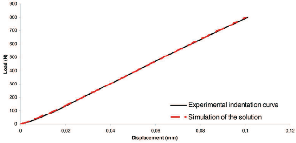
FIG. 9: Comparison between experimental and numerical indentation curves for the carbonitrided not quenched C18 steel. (a): substrate (b): surface
