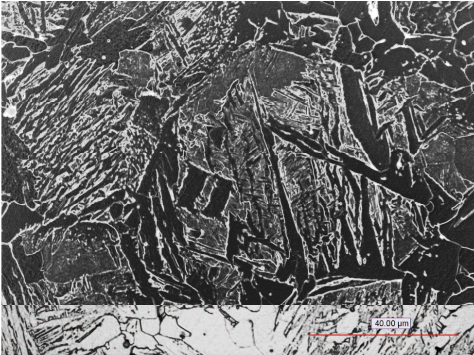
FIG. 10: microstructure of the carbonitrided C18 steel. (a) : Microstructure of the substrate (b) : Microstructure of the surface
