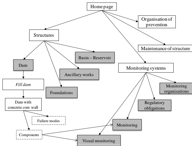
Figure 2. Partial view of the fields of the SANBA-dom tool
