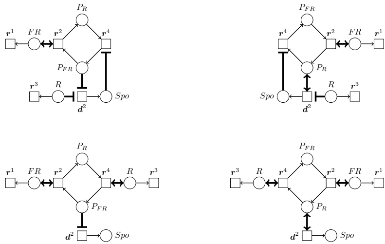
Figure 7: From S_4 , four minimal catalytic conformal networks \mathcal{P}_{S_4} result, all with priority relations \mathcal{O}_4 = \{(\mathbf{r}^2 > \mathbf{r}^1), (\mathbf{r}^4 > \mathbf{r}^3)\} .
