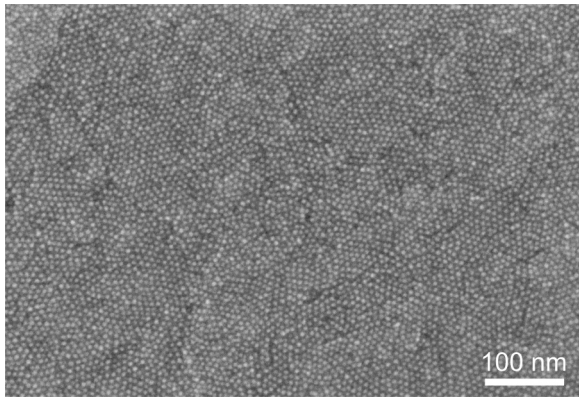
FIG. 11. Large-scale SEM image of PbSe/CdSe heteronanocrystals transferred by the Langmuir-Blodgett technique onto a gold-terminated Si(111) surface. The sample was observed after its characterization by synchrotron radiation. The initial dimensions of the heteronanocrystals were: core diameter of 4.4 nm and shell thickness of 1.1 nm.
