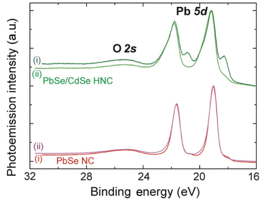
FIG. 9. (Color online) Evolution of the high-resolution Pb 5d and O 2s core-level spectra of PbSe nanocrystals (diameters: 9.3 nm) and PbSe/CdSe heteronanocrystals (core size: 5.3 nm and shell thickness: 2.0 nm) under illumination at 95 eV. Spectra (i) and (ii) correspond to a brief and longer illumination, respectively.
