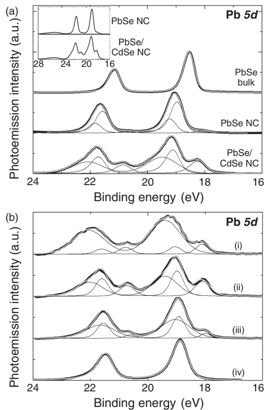
FIG. 3. (a) Background subtracted high-resolution Pb 5d core-level spectra of bulk PbSe, PbSe nanocrystals (diameters: 9.3 nm), and PbSe/CdSe heteronano-crystals (core sizes: 5.3 nm and shell thicknesses: 2.0 nm). The thin lines correspond to fits obtained with the parameters given in Table I. The photon energy was set at 95 eV. Inset: background subtracted Pb 5d core-level spectra of the PbSe nanocrystals and PbSe/CdSe heteronano-crystals observed on a wider energy range to show a broad and small peak around 25 eV. (b) Evolution of the line shape of the Pb 5d core level during the surface preparation of bulk PbSe. Spectrum (i) corresponds to a surface treated with a soft Ar sputtering, whereas, spectrum (iv) was measured after three cycles of sputtering and annealing. All spectra were measured at room temperature.
