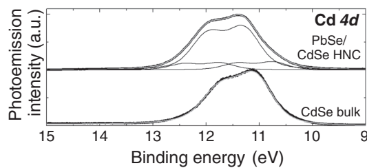
FIG. 5. Background subtracted high-resolution Cd 4d core-level spectra of PbSe/CdSe heteronanocrystals (core size: 5.3 nm and shell thickness: 2.0 nm) and bulk CdSe, obtained with photon energies of 95 and 90 eV, respectively. The thin lines correspond to fits obtained with the parameters given in Table I. Both spectra were measured at room temperature.
