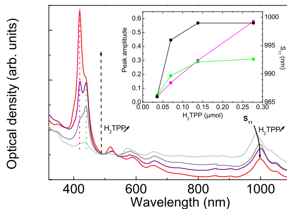
Figure 5: (color online) Absorption spectra of H 2 TPP@SWNT micellar suspensions for various amounts of H 2 TPP (the water volume is 2.5 mL) : 0.04 μmol (light gray), 0.07 μmol (gray), 0.14 μmol (purple), 0.28 μmol (red). The DCM/water volume ratio is kept constant (34%). The spectra were vertically translated in order to compensate for the background scattering at 490 nm. Inset : Maximum value of the absorption bands of free H 2 TPP at 420 nm (pink), of stacked H 2 TPP at 438 nm (green) and position of the S 11 transition of (6,5) SWNTs (black, right scale) as a function of the added H 2 TPP amount. (Figure taken from Ref.[24]).
