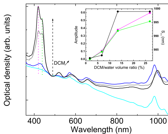
Figure 4: (color online) Absorption spectra of H 2 TPP/SWNT suspensions obtained for various DCM/water volume ratio : 2% (light blue), 7% (blue), 13% (gray) and 27 % (black). The quantity of H 2 TPP is constant (0.14 μmol) and the water volume is 2.5 mL. The spectra were vertically translated in order to compensate for the background scattering at 490 nm. Inset : Maximum value of the absorption bands of free H 2 TPP at 420 nm (pink), of stacked H 2 TPP at 438 nm (green) and position of the S 11 transition of (6,5) SWNTs (black, right scale) as a function of the DCM/water volume ratio. (Figure taken from Ref.[24]).
