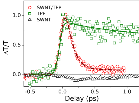
Figure 12: (color online) Normalized transient transmission dynamics measured in a degenerate configuration in resonance with the Soret band in free H 2 TPP in micelles (green squares), in H 2 TPP@SWNT in micelles (red dots). Same measurement at 438 nm in bare SWNTs in micelles (black triangles) which allows to check that the intrinsic signal from SWNTs is negligible at this wavelength (from Ref. [28]).
