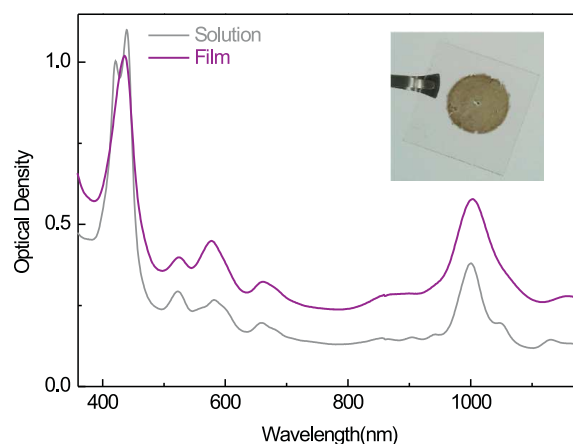
Figure C.19: (color online) Absorption spectrum of a film of H_2TPP@SWNT together with the absorption spectrum of the suspension used to make it. Inset : picture of the film deposited on a quartz substrate.
