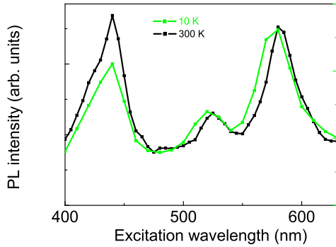
Figure 10: (color online) PLE spectra of (6,5) nanotubes in a thin film of H_2TPP@SWNTs (detection : 1005 nm) at room temperature (black line) and 10 K (green line).
