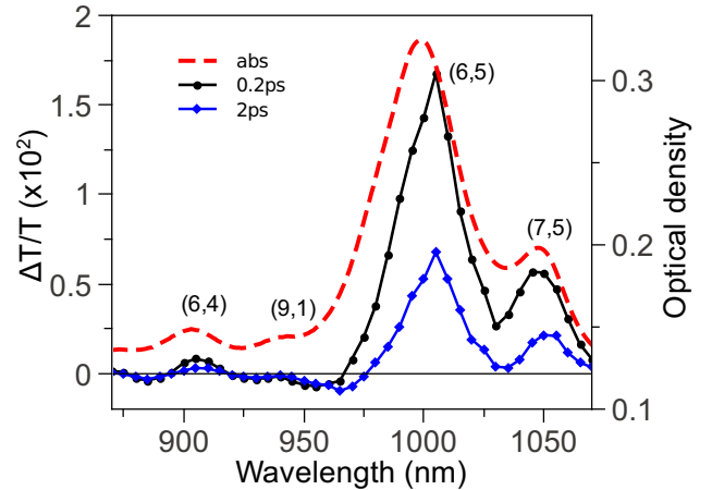
Figure 13: (color online) Transient absorption spectrum of H 2 TPP@SWNT for a pump at 445 nm in resonance with the Soret band and a broadband probe in the NIR. The pump-probe delay is 0.2 ps (black dots) and 2 ps (blue squares). Right axis : linear absorption of the sample (dashed line). The majority chiral species is indicated in parenthesis for each line. (Figure inspired from Ref. [28]).
