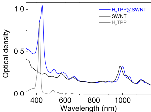
Figure 3: (color online) Absorption spectrum of a micellar suspension of Co-MoCat nanotubes (black line), a micellar suspension of H 2 TPP (gray line) and a suspension of functionalized nanotubes (blue line).
