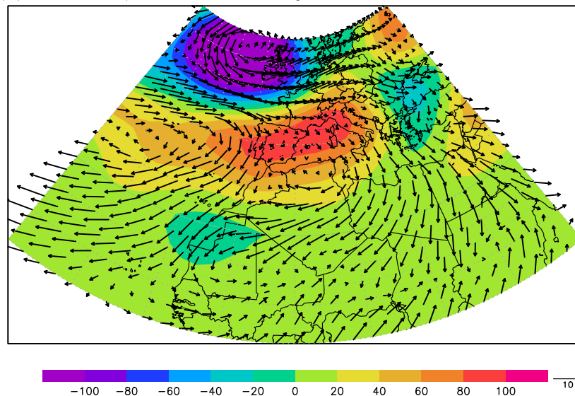
Figure 2. Circulation during the “maritime” and “heat low” phases of Fennec IOP. (a) Mean anomalies of 300 hPa geopotential height and absolute 925 hPa winds from ERA-Interim data during 1–11 June 2011. (b) As Figure 2a but for 13–25 June 2011.
