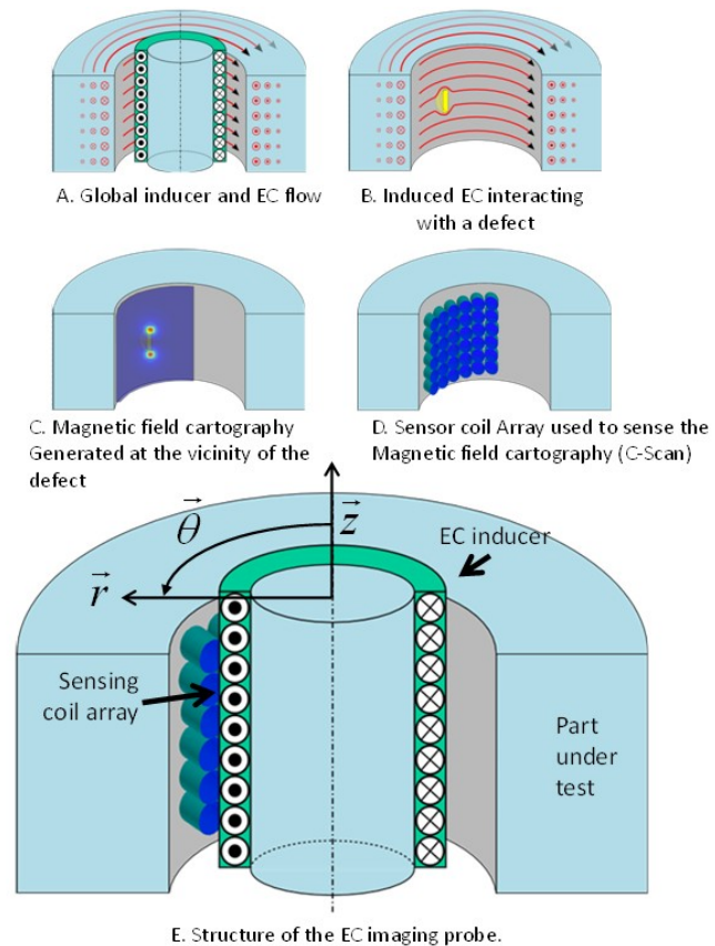
Figure 1. Structure and basic principle of the EC imaging probe.
