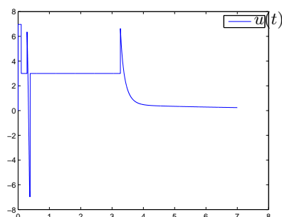
Fig. 3. Evolution of the control u .
