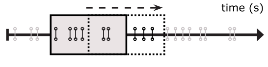
Fig. 6. Sliding time window over a stream of appearing links.
