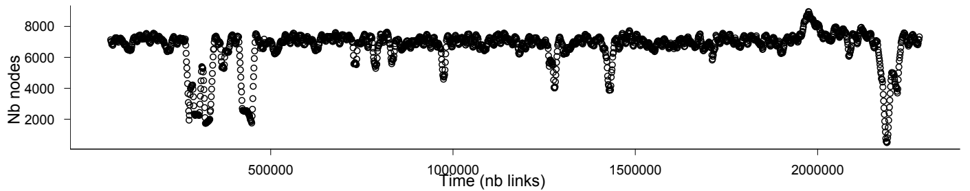
Fig. 9. Github: number of nodes in a sliding window of 10,000 links, for each set of 1000 links.
