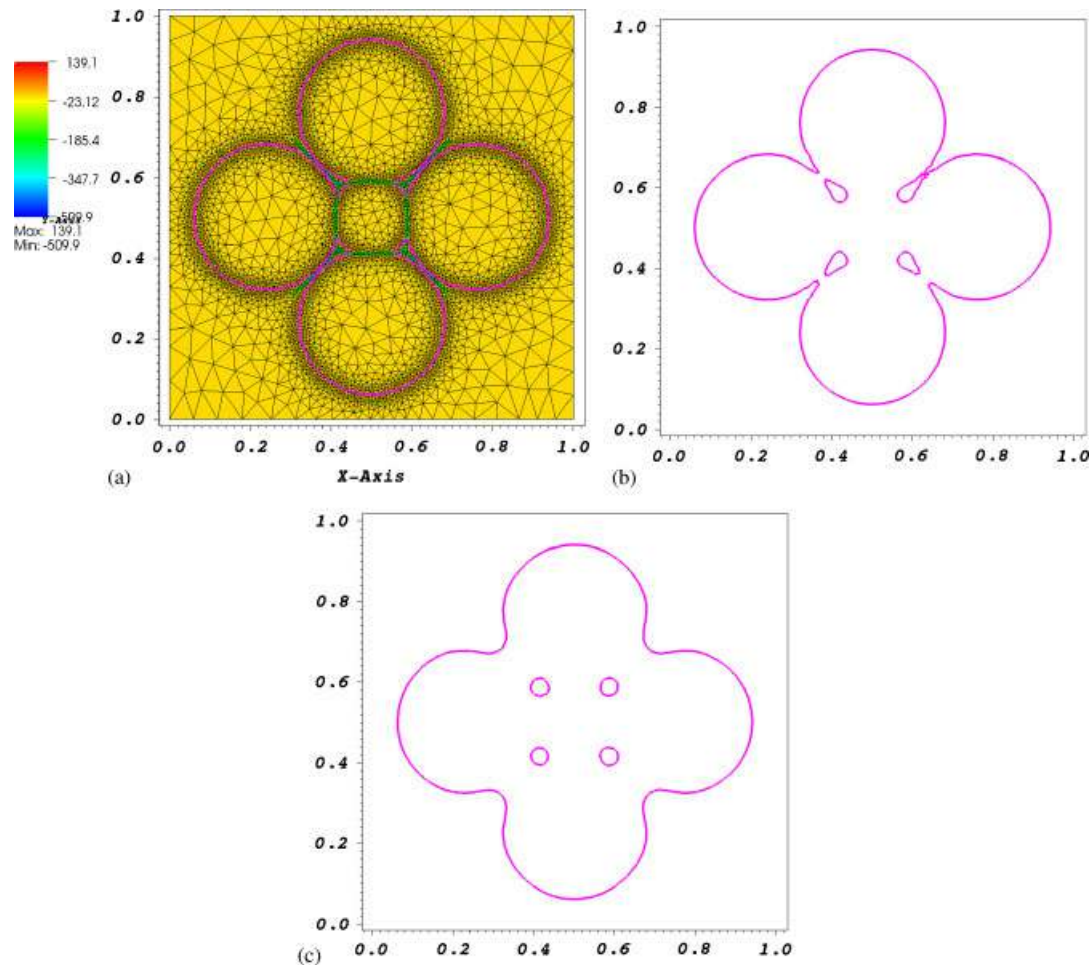
Figure 14. Change in 5 grains under surface diffusion (two-dimensional case, C_0=10^{-7} , \Delta t=5.0 \times 10^{-3} ). (a) Adapted mesh and curvature, and (a)–(c) Interface \{\phi_n=0\} (solid line). (a) t=0 ; (b) t=0.1 ; and (c) t=5 .
