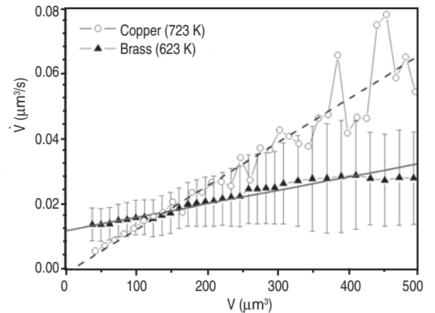
Figure 8. Growth rate of voids as a function of volume. Voids in OFHC copper obey Equation 3, while growth-rate of voids in brass has a positive intercept.
