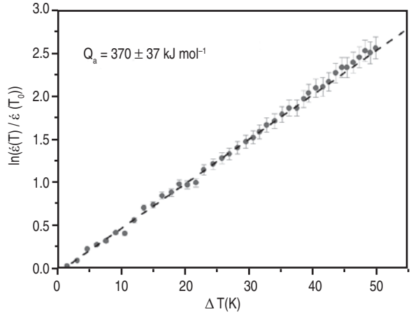
Figure 3. Variation of normalized strain rate as a function of temperature difference \Delta T , along the gauge length of the specimen. T_0 represents the lowest temperature in the investigated volume and \dot{\epsilon}(T_0) the corresponding strain-rate. The slope of the fitted line is proportional to the apparent activation energy of steady-state creep (see Equation 2).
