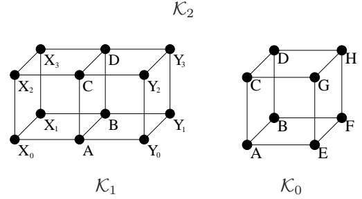
Figure 13: \mathcal{K} -neighborhoods for 2-cliques ( \mathcal{K}_2 ), 1-cliques ( \mathcal{K}_1 ), and 0-cliques ( \mathcal{K}_0 ). A voxel is represented by its central point.
