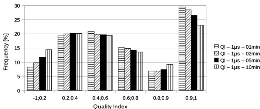
FIG. 2. QI distribution of 40 000 ground targets selected around the Nîmes radar on 20 Sep 2011 for 12 h. The horizontal hatching, diagonal hatching, solid black, and vertical hatching correspond to a 1-, 2-, 5-, and 10-min sampling time, respectively.
