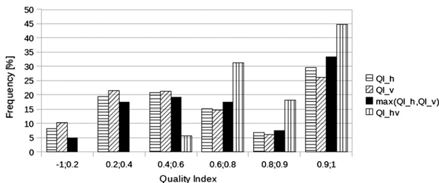
FIG. 11. QI distribution of 40 000 ground targets from 20 to 21 Sep 2011 for 12 h. The horizontal hatching, diagonal hatching, black color, and vertical hatching correspond to QI_h , QI_v , \max(QI_h, QI_v) , and QI_{hv} , respectively.
