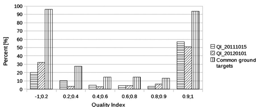
FIG. 3. QI distribution of 11 000 ground targets selected around the Trappes radar for 24 h. The horizontal hatching corresponds to the \text{QI}_{2011-10-15} of 15 Oct 2011, the diagonal hatching to the \text{QI}_{2012-01-01} of 1 Jan 2012, and the vertical hatching to the percentage of pixels that are present in the same class at each of the two time sequences considered.
