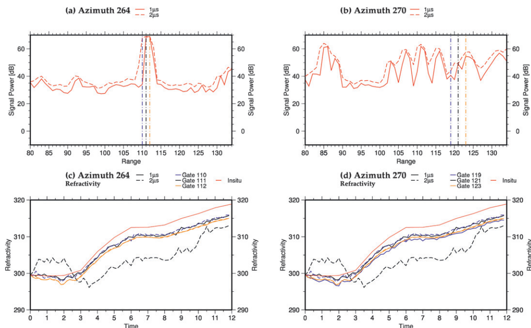
FIG. 7. (top) Range profiles of signal power (dB; red) as a function of range at azimuth (a) 264° and (b) 270°. (bottom) The 12 time series of the refractivity measurement for the in situ parameters (red) and for (c) radar gates 110 (blue), 111 (black), and 112 (orange) in the azimuth 264° and (d) radar gates 119 (blue), 121 (black), and 123 (orange) in the azimuth 270°. Solid and dashed lines indicate respectively a 2- \mu s and 1- \mu s transmitter pulse duration on 20 Sep 2012 with the Nîmes radar.
