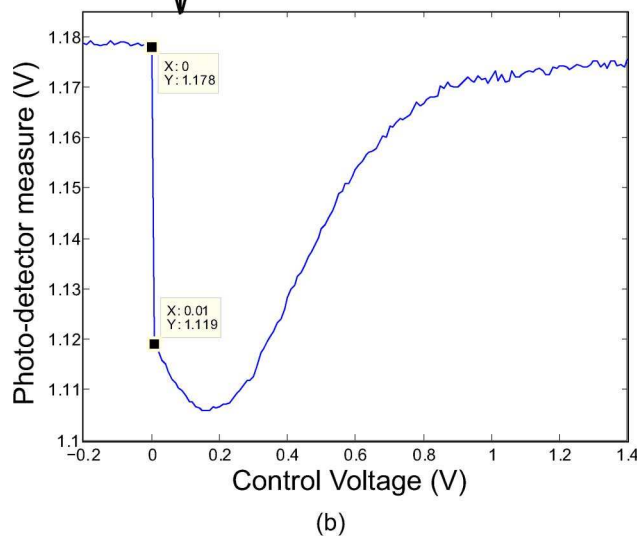
Fig. 5. (Color online) Variation of intensity (a) I_h + I_v and (b) zoom at a specific voltage range of the curve I_h + I_v .
