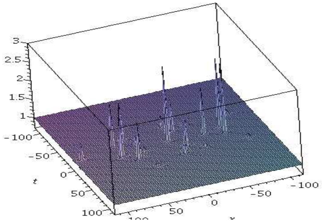
Figure 4: Solution of NLS, N=6 , \tilde{a}_2 = 10^8 , 3 rings with respectively 5, 10, 5 peaks with in the center one peak.
