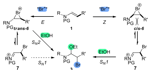
Scheme 3. Mechanistic Proposal
