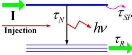
FIG. 1. Sketch of the simplified carrier dynamics model in injection-locked QCLs.
