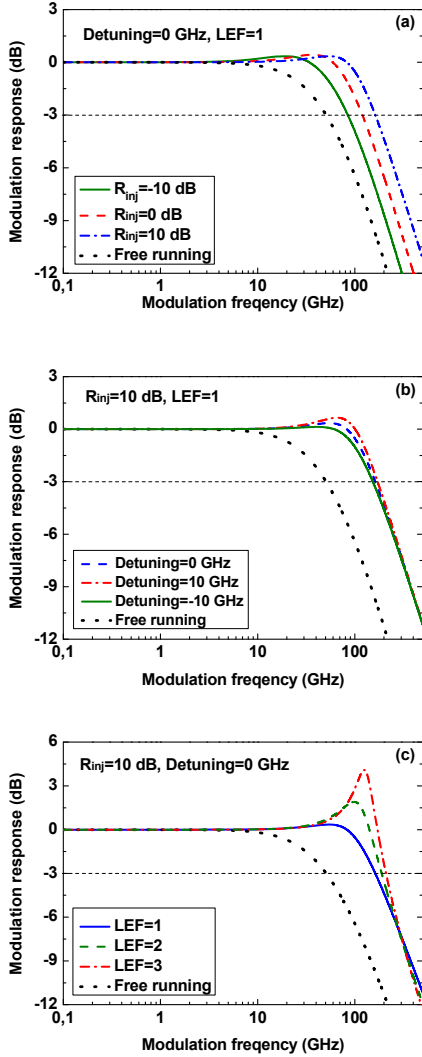
FIG. 3. IM response of optical injection-locked QCLs for fast carrier removal rate ( \tau_r = 0.21 ps) as a function of (a) Injection ratio at zero detuning with LEF=1, (b) detuning frequency at R_{inj}=10 dB with LEF=1, and (c) LEF at zero detuning with R_{inj}=10 dB.
