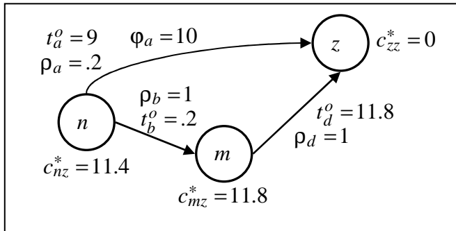
Fig. 2. Small instance.
