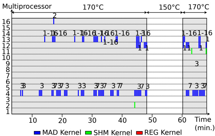
Figure 4. Error localisation in function of time and temperature on the GPU C870 number 1. Single numbers indicate the faulty SP unit. Range numbers such as 1-16 corresponds to a vector error.
