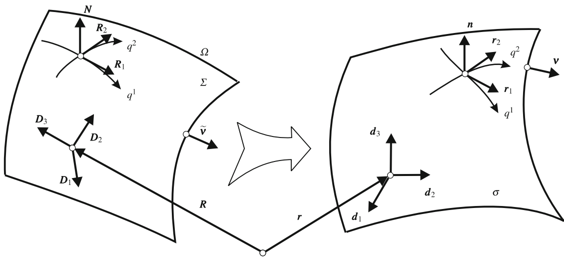
Fig. 2 Deformation of the micropolar shell
