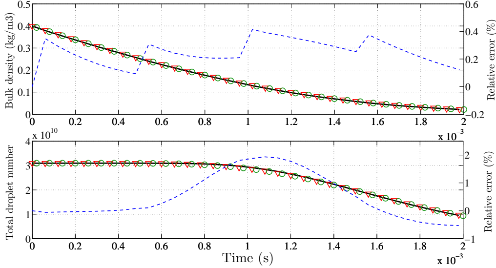
Figure 2: Spray bulk density (top) and total droplet number (bottom) evolutions / CEDRE : \circ , SAP1 : \nabla , SAP1 error : --- , Analytic solution : Black
